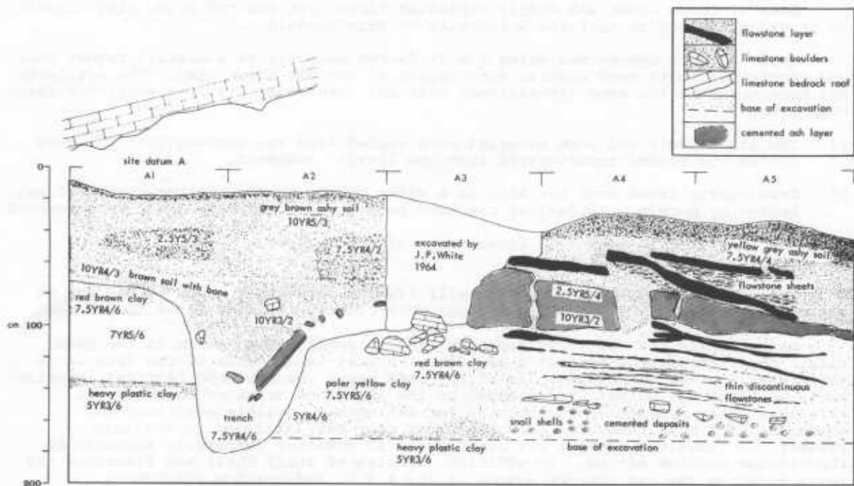
Figure 3: Section diagram of north face of squares A1 to A5, running east from site datum A, as recorded during 1979 excavations.
