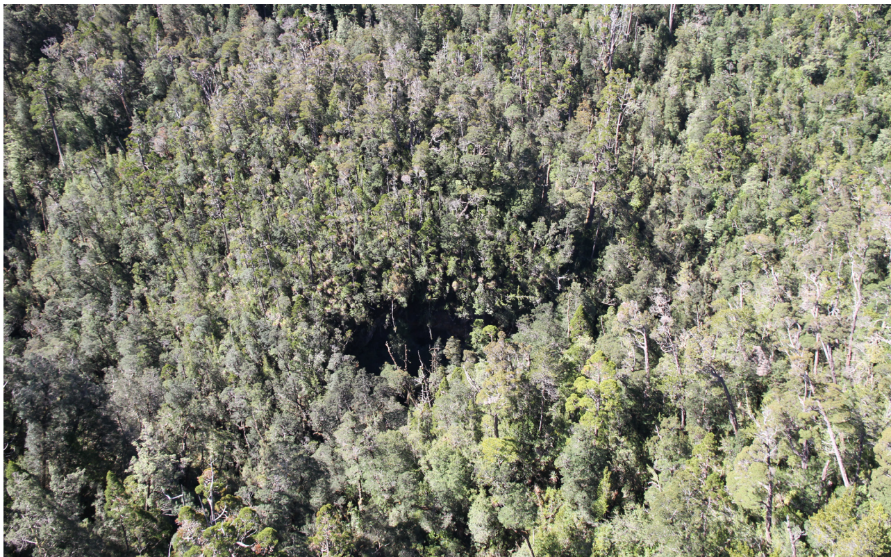
Figure 4. Aerial view of the deepest point of the Forest Hills Depression. The apparent cavity at the centre of the image is a 20 m high overhanging cliff directly above Forest Hills Cave (see Figure 15). In this image the point of entry to the cave is concealed by vegetation (Photo by Rolan Eberhard).
