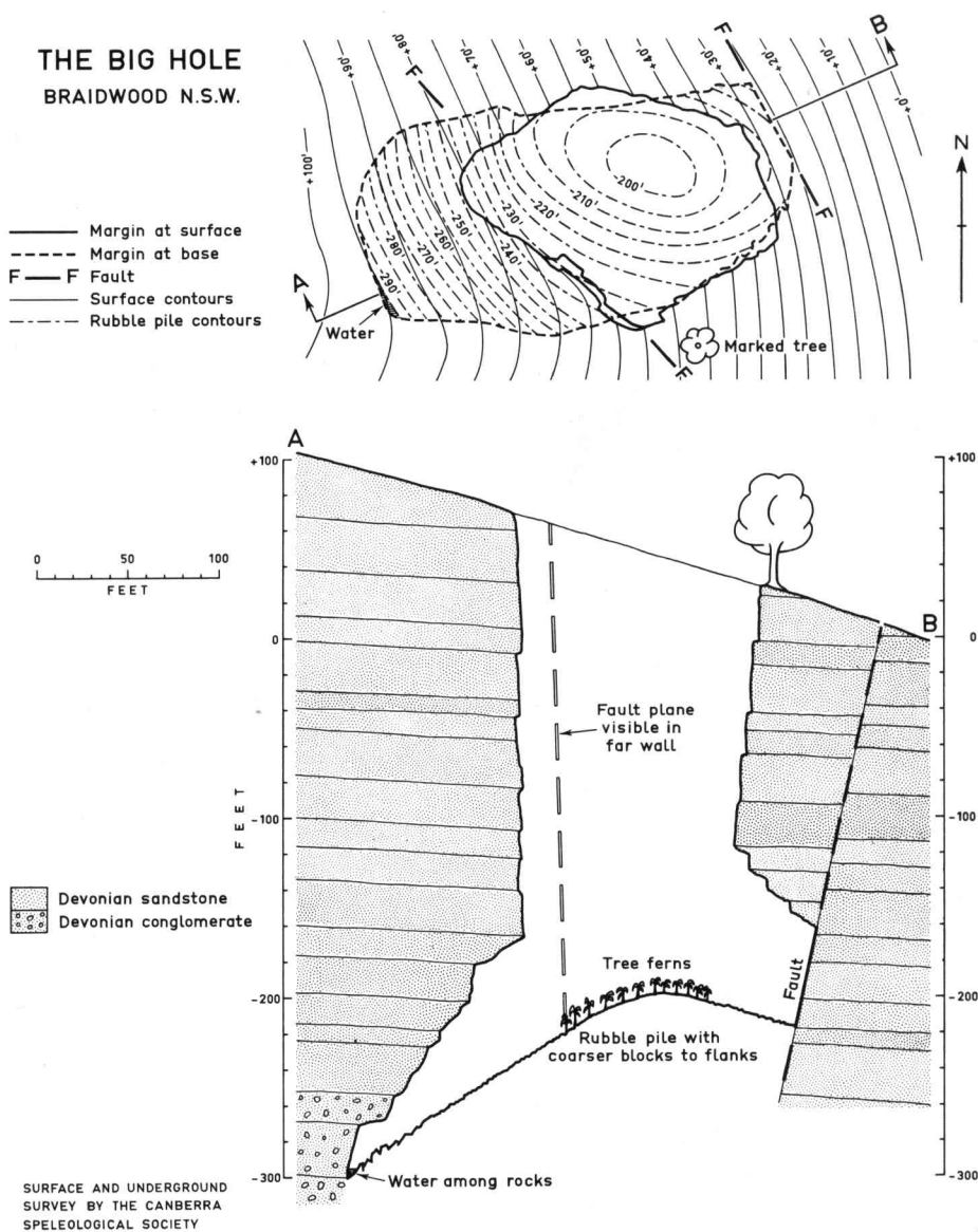
Figure 1. A revised plan and section of the Big Hole. The datum for heights is arbitrary.
