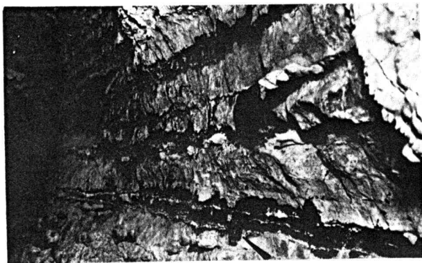
PLATE 5. Limestone wall in Cave No. 41 showing crystal wedging by gypsum. Darker areas have undergone recent spalling. Arrow indicates flash bulb for scale.
