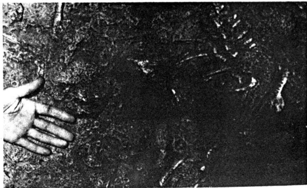
PLATE 2. Vertebrate skeleton embedded in underside of flowstone sheet in Deep Hole.
