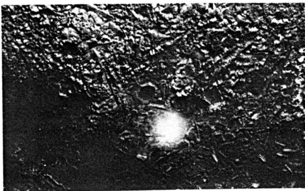
PLATE 3. Broken stalactites embedded in underside of flowstone sheet in Deep Hole. Light spot is about 8 cm in diameter.
