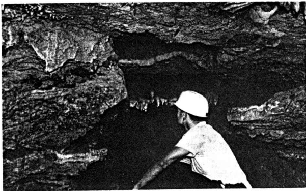
PLATE 1. Two lower flowstone sheets in Deep Hole.
