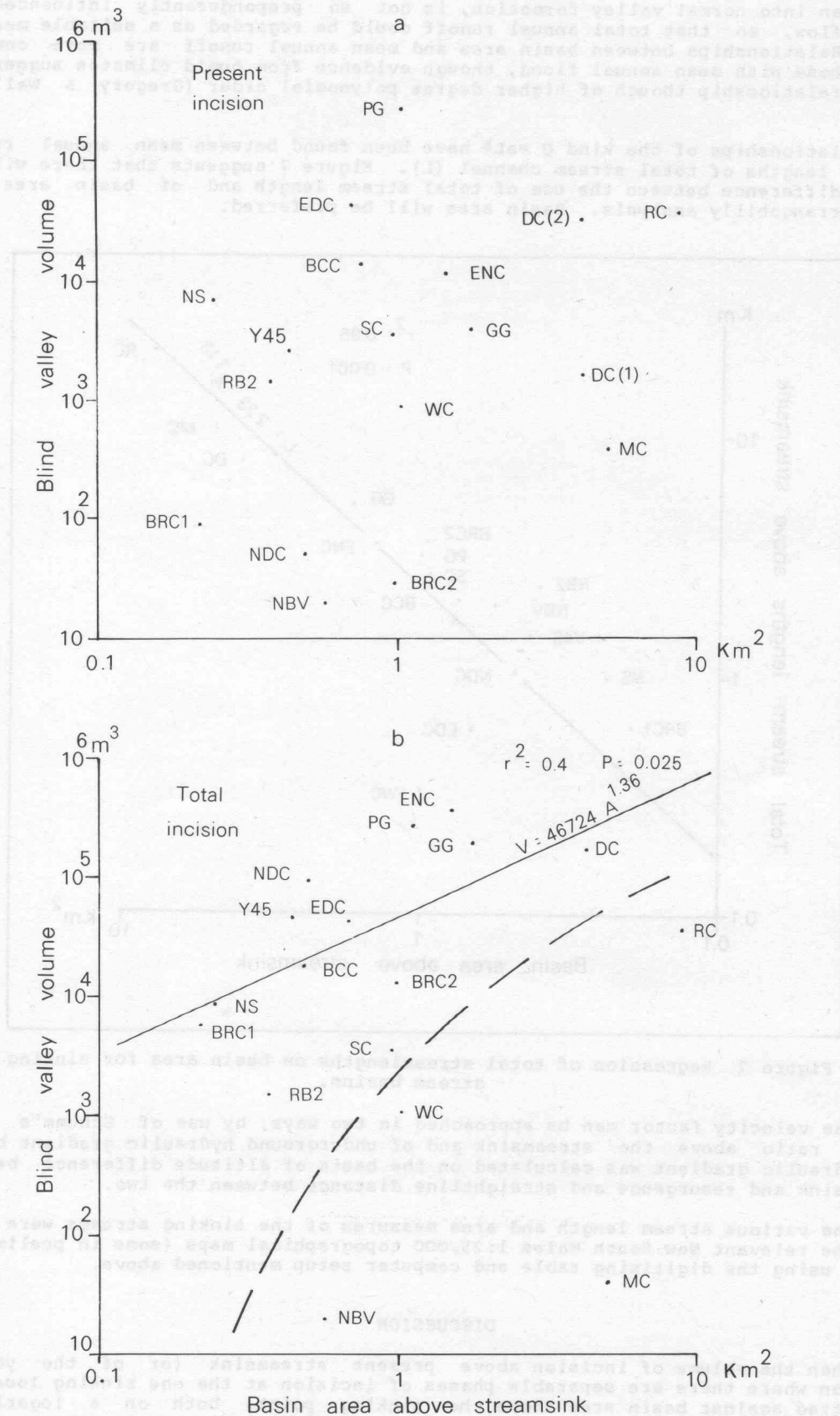
Figure 8 Scatter diagrams of blind valley volume against basin area of sinking streams. In 8b, the regression is for a restricted set of blind valleys, excluding the four below the dashed line.
