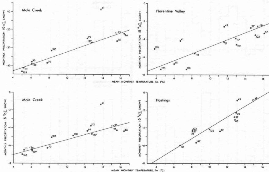
Figure 7. Statistical relationships between \delta^{18}\text{O} (SMOW) values and mean monthly temperatures at the three stations as well as the relationship of \delta\text{D} SMOW values and mean monthly temperatures at Mole Creek.
