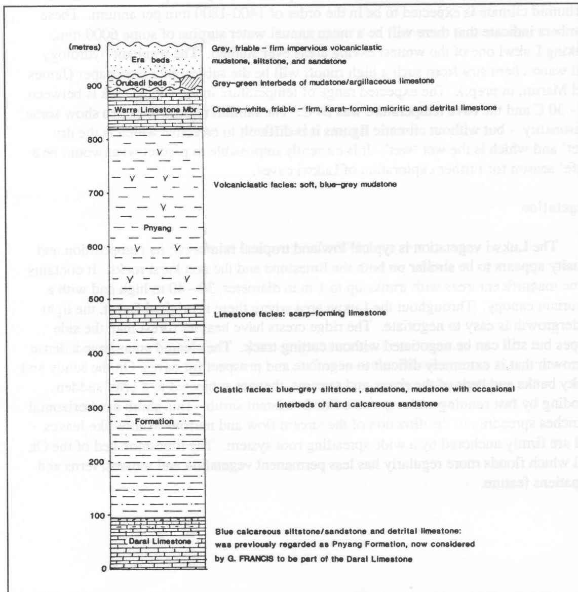
Figure 2. Neogene stratigraphic relationships in the Ok Tedi region.
