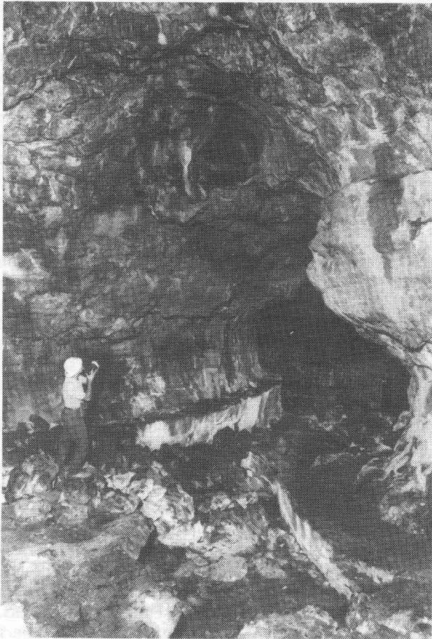
Plate 6: Taylor Cave. The prominent 'pavements' (1 and 2) are evidence of an extended period of constant rate of flow. Solidification has been greatest at the apex of convexity, as in a fluvial river. There is a cylindrical opening (3) in the roof above the figure. The location of this opening suggests that some lava ponded in the Death Adder depression (in alignment to the north), may have drained back into the tube through this conduit.
