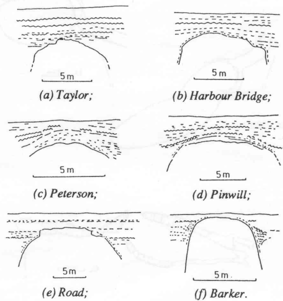
Figure 6: Cave entrance structures showing thickening of roofs by successive surface flow units. Flow units are indicated by wavy lines for recognised flow unit surfaces. Other near-horizontal lines are major vesicle zones. Diagram: P.J. Stephenson.
