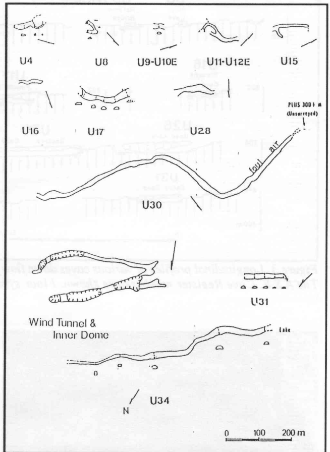
Figure 2: Maps of selected caves with some cross sections. In all cases, lava flowed through the cave passage from left to right. Localities - see Figure 1; cave names - see Figure 3. Cave U11-12E is Greeley Cave (Atkinson et al., 1975); The Wind Tunnel and Inner Dome plans are shown (Operation Raleigh & M Godwin, 1989). The 1987 extension of Bayliss Cave is not shown.
