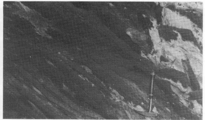
Plate 7: Multi-layered lining in Pinwill Cave. Up to fifteen layers are exposed at this location. Photo: V.G. Atkinson.
