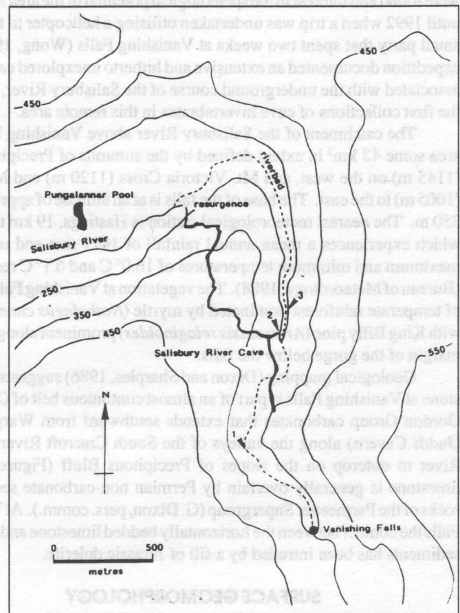
Figure 2. Salisbury River Cave. Surveyed with Suunto compass and clinometer read to the nearest 1.0^\circ and 30 m fibreglass tape to the nearest 0.1 m. Passages upstream of Gorge Entrance were surveyed by pace and compass. Fossil or intermittently active inflow points are indicated by arrows: 1 = Downstream limit of flow on 16/4/92, 2 = Gorge Entrance, 3 = Bushwalkers Cavern.
