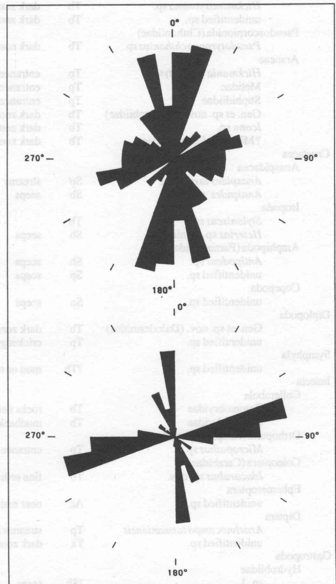
Figure 5. Rose diagrams.
