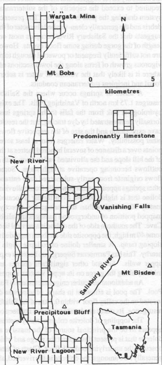
Figure 1. Interpretive geological map showing the possible extent of late Ordovician Gordon Group carbonates in the Mt. Bobs-Precipitous Bluff area. After Dixon & Sharples (1986).
