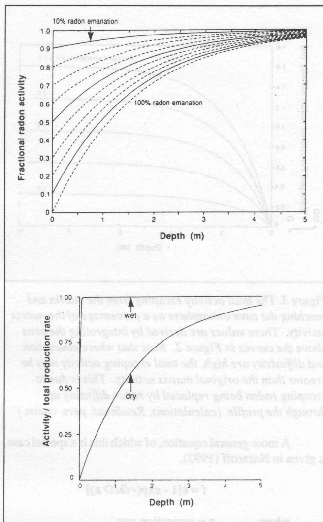
Figure 2. a) Fractional radon activity curves for U-238 series for different emanation rates, redrawn from Readhead (1984). Calculations assume the sediment is dry. The radon diffusion coefficient was taken as 5.4 \times 10^{-2} , which was calculated for building sand with a density of 1.4 \text{ g cm}^{-3} , with a 39% porosity filled with air with a 4% moisture content (Tanner, 1964)
