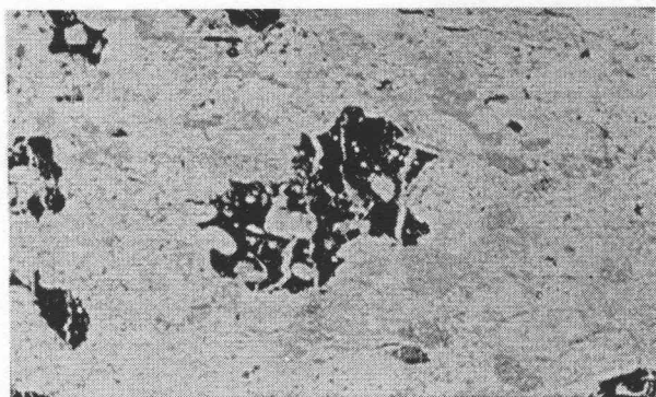
Figure 3 Pyrite in palaeokarst breccia, Lune River Quarry, Tasmania. Thin section. Transmitted light, Crossed nicols. Pyrite forms opaque masses around large original clasts. Long axis of central pyrite mass is 5 mm.
