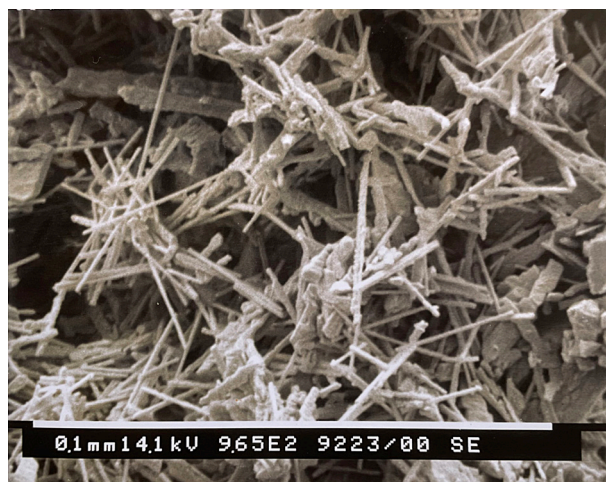
Figure 11. Moonmilk from Mammoth Cave (J13) Jenolan NSW. Sample contained both calcite and aragonite. Fibrous calcite strands are approximately 1.5\mu\text{m} thick. Image by Brian England
