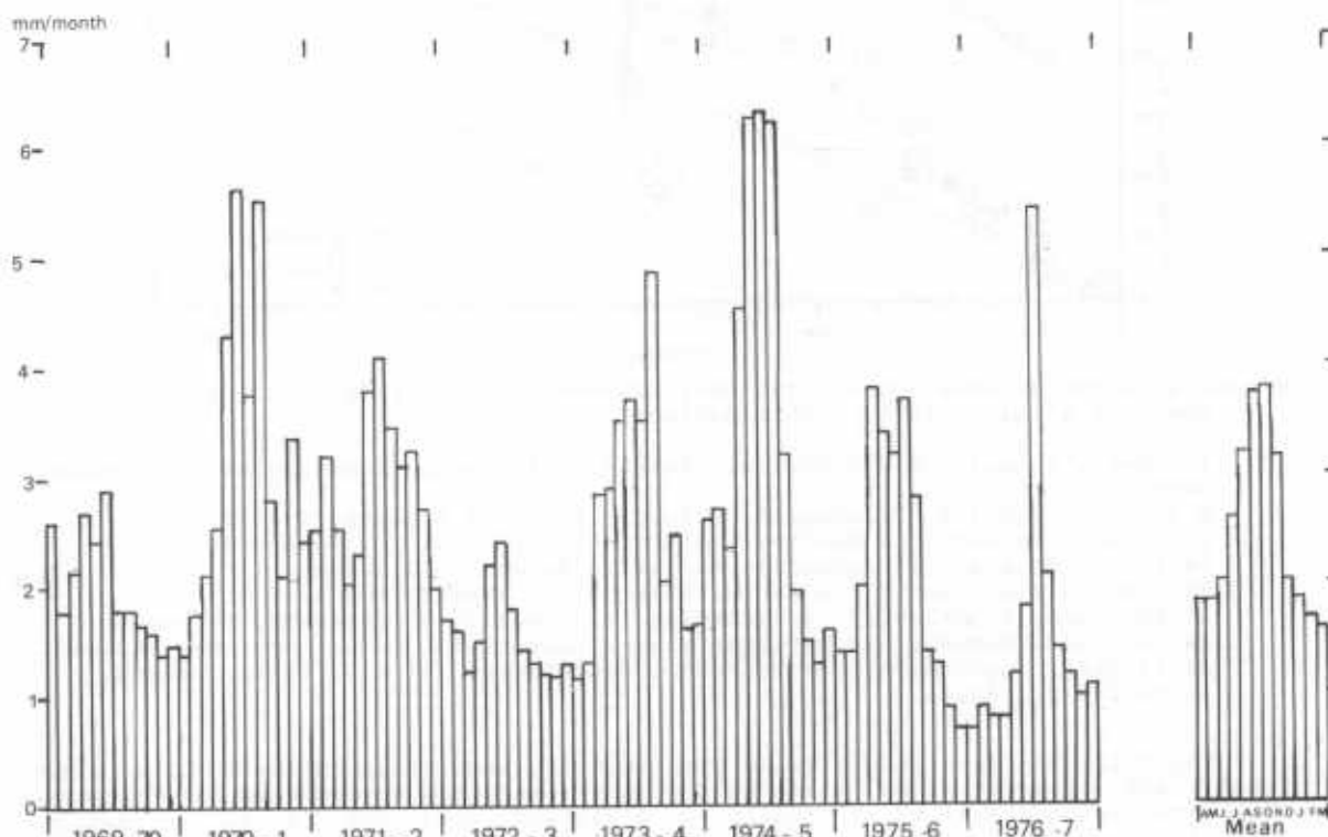
Figure 17 Monthly carbonate load from exposed karst, Coleman Plain, 1969-77
