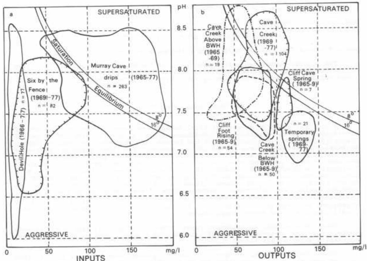
Figure 13 Picknett graphs to show solutional capacity of (a) input and (b) output streams, Coolleman Plain
