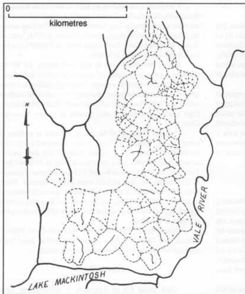
Figure 3: Drainage divides in the Polygon karst
