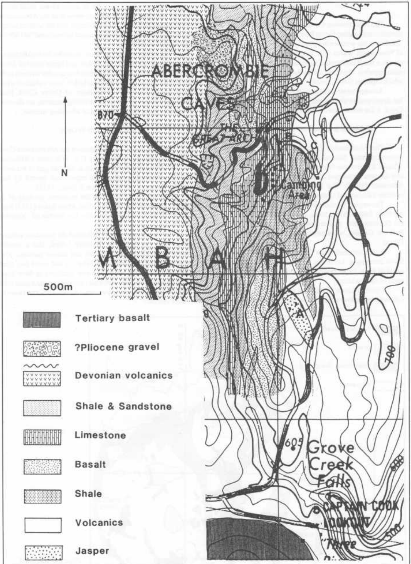
Figure 3: Geology of the Abercrombie Caves Reserve. Based on Morrissey and Green n.d. Field revision by the author 1990.
