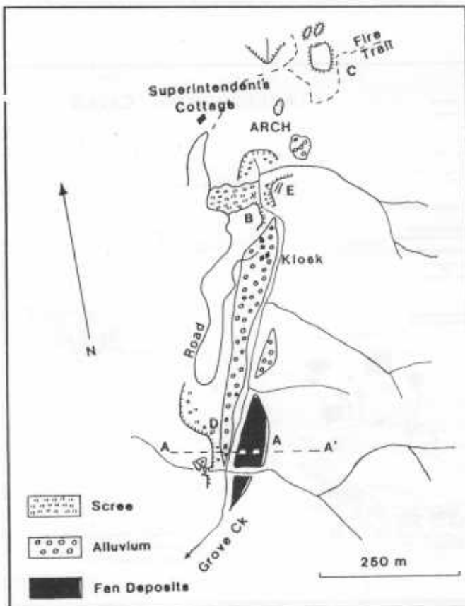
Figure 5: Surficial Geology.
