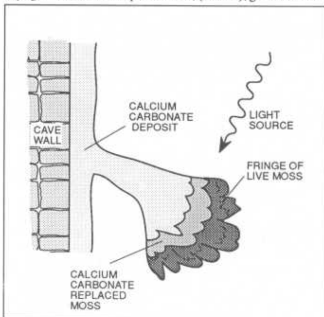
Figure 2. Simplified form of a phototropic phytospeleothem.
